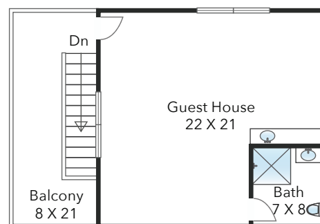
Upper Level Garage / Guesthouse
